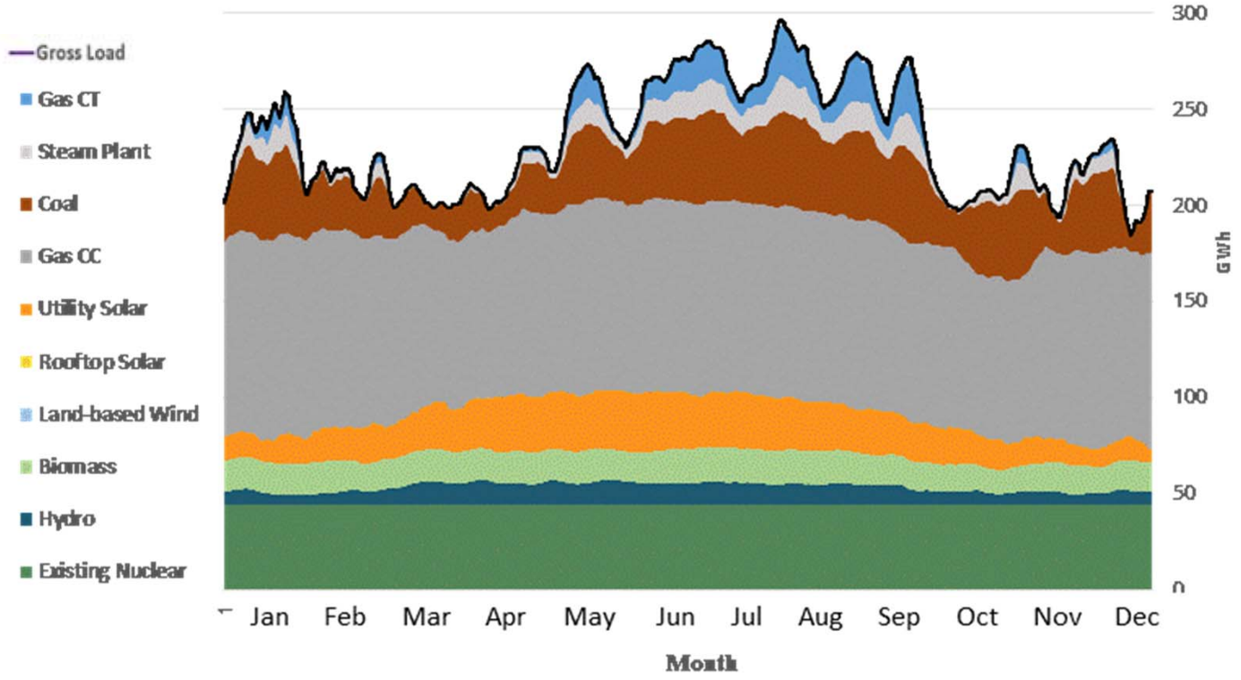
Daily Generation and Load (GWh) GPC Existing Sources 2022
